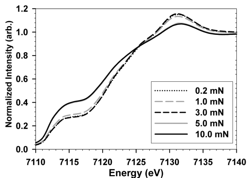
FIGURE 2. Passivation of nitrate as a function of concentration is shown in the Fe K-edge XANES of NZVI aged with varying concentrations of nitrate (0.2–10 mN) showing bimodal retardation of NZVI oxidation by water over 1 month. The higher concentrations retain an average particle oxidation state close to the original particle, with 5 mN and 10 mN sharing identical shape and position, whereas the lower concentrations of 0.2–3 mN advance to higher oxidation.
