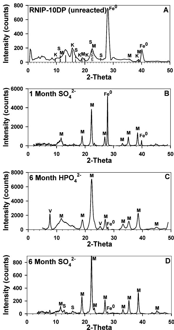
FIGURE 5. (A–D). XRD patterns of unreacted and exposed NZVI, in 10 mM sulfate and phosphate. (A) = dry-unreacted RNIP showing the presence of mostly Fe 0 , with some magnetite and iron sulfate species (schwertmannite and mikasaite). (B) = NZVI aged for 1 month in sulfate, where the sulfate species from (A) have disappeared and magnetite has increased in proportion to Fe 0 . (C) = 6 month aged in phosphate; vivianite peaks appear at ~7° and 25° 2θ. (D) = 6 month aged in sulfate; indications of schwertmannite arise as peaks at ~13° and 16° 2θ. Species symbols and line styles in (A) indicated in parentheses: Fe 0 is labeled as such, M = magnetite (dotted), S = schwertmannite (dashed), K = mikasaite/Fe 2 (SO 4 ) 3 (solid line). Vivianite only appears in (C) and is represented by V. (A) has been cropped to show more detail below 800 counts. The peak at ~28° 2θ has a maximum value of ~1000 counts.
