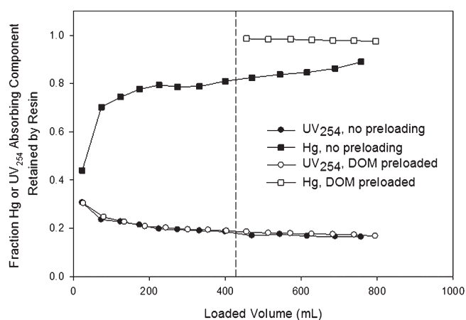
Figure 2. Mercury retention and DOM retention (as measured by the UV absorbance of DOM components that absorb at 254 nm) for a system without DOM preloading of the resin and a system with DOM preloading of the resin. The system without preloading (0.45 nM Hg, 10.6 mg DOM L -1 , 100 μM sulfide) was run as a standard chromatography experiment with the mercury-containing solution started at a loaded volume of 0 mL. The preloaded system consisted of DOM preloading (9.8 mg DOM L -1 , 100 μM sulfide) up to a volume of 428 mL (dashed vertical line) at which time an identical solution equilibrated with mercury (0.40 nM) was loaded on to the resin.
